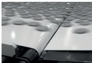
Standard TPU series Food. Highly resistant to animal and vegetable oils and fats, no cracks, high level of hygiene. High resistance to cut and abrasion. Fabrics with low capillarity (Wicking Test G11-FDA 2011).
