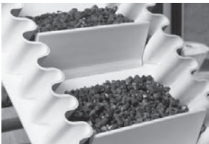
Esport series Food. Excellent resistance to vegetable oils and fats. For roller troughed conveyors and bucket elevators. Conveyance of organic materials: food, seeds, compound fodders, waste.
